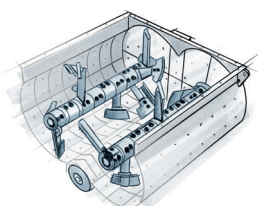
Twin shaft mixer
