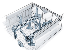
Twin shaft mixer
